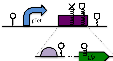
Figure 35: Promoter regulating the production of an engineered composite sequence that includes RNA and protein stability elements at its 3' end, as well as an internal site for protease cleavage, as well as the expansion of the composite to show it contains a ribosome entry site, coding sequence, and other omitted details. Single residue locations of interest are indicated for the DNA (before the promoter), RNA (after the ribosome entry site), and protein (in the CDS).
