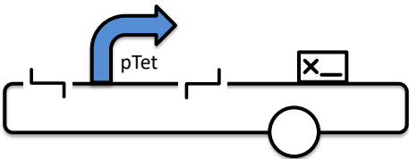
Figure 30: Promoter pTet stored in a circular plasmid. The promoter is prepared for being cut out of the plasmid: it is preceded by a 5' sticky end restriction site and followed by a 3' stick end restriction site. In addition, the plasmid has been bar-coded with a signature and has its origin of replication marked.
