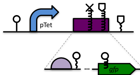
Figure 34: Promoter regulating the production of an engineered composite sequence that includes RNA and protein stability elements at its 3' end, as well as an internal site for protease cleavage, as well as the expansion of the composite to show it contains a ribosome entry site, coding sequence, and other omitted details. Single residue locations of interest are indicated for the DNA (before the promoter), RNA (after the ribosome entry site), and protein (in the CDS).
